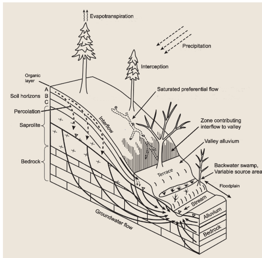
Figure 1. Cross-section of a typical forested hillslope over weathered bedrock showing hydrologic processes and flow paths. Most rainwater reaches streams by long subsurface routes. Only near-channel areas with proximal water tables produce overland flow during storms because of soil saturation.
